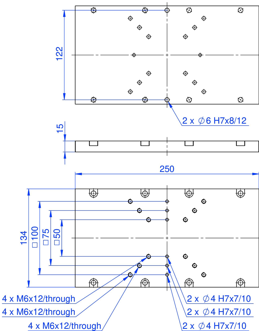
V-857.TT1, dimensions in mm
