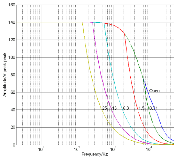
E-617: Operating limits (open loop) with various capacitive loads, capacitance values in \mu\text{F}
